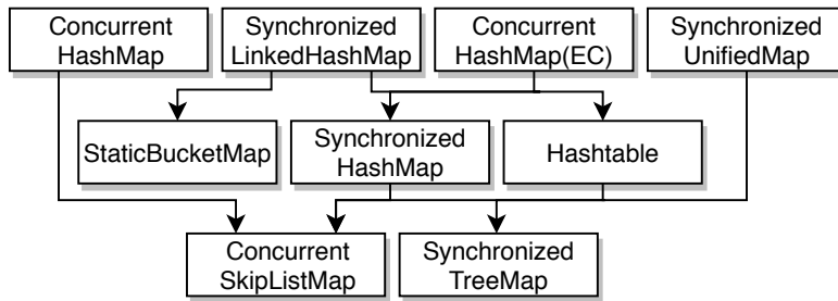
Fig. 3 Order of dominance between the thread-safe Map implementations on server . Arrows point from the dominating collection to the dominated one.
