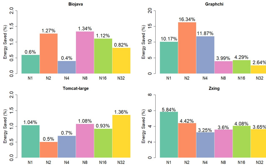
Fig. 2 Percentage of Energy saved by CT+ among the different software systems.
